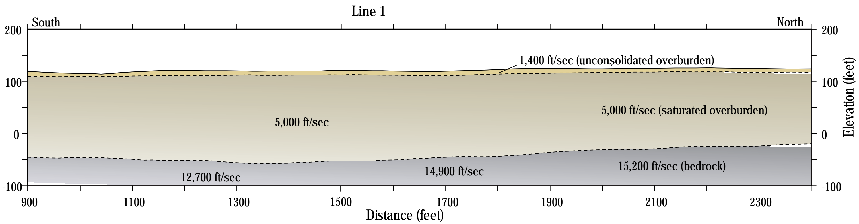
Figure 7 - Seismic Refraction Cross-Section Former Raytheon Facility - Wayland, MA
